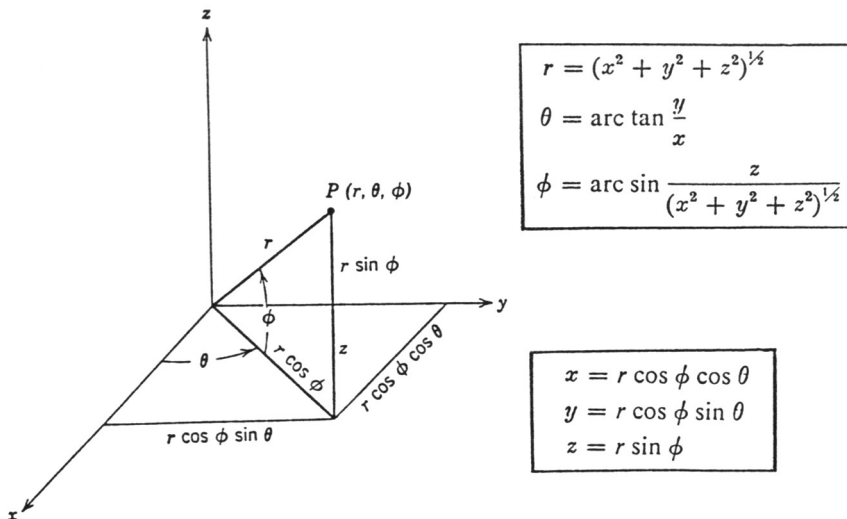
Relationships among Cartesian and spherical coordinate variables.
